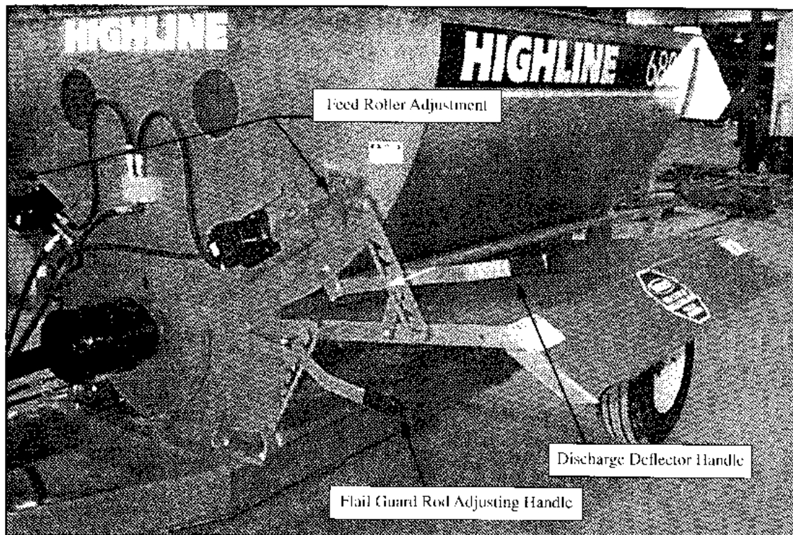
Figure 1 Manual Controls
